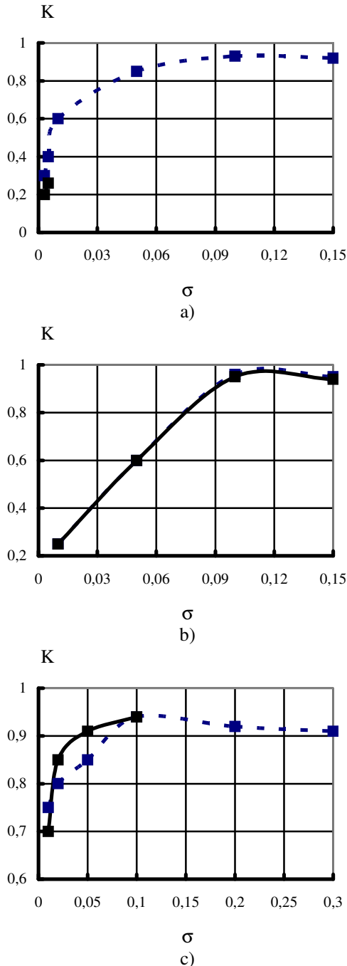
Fig. 3. Dependencies of correct recognition probability on the influence parameter \sigma of a neural network for three modes of GTE: a) m1, b) m2 and c) m3 (continuous lines – \vartheta=0,05 , dotted lines – \vartheta=0,03 ).
