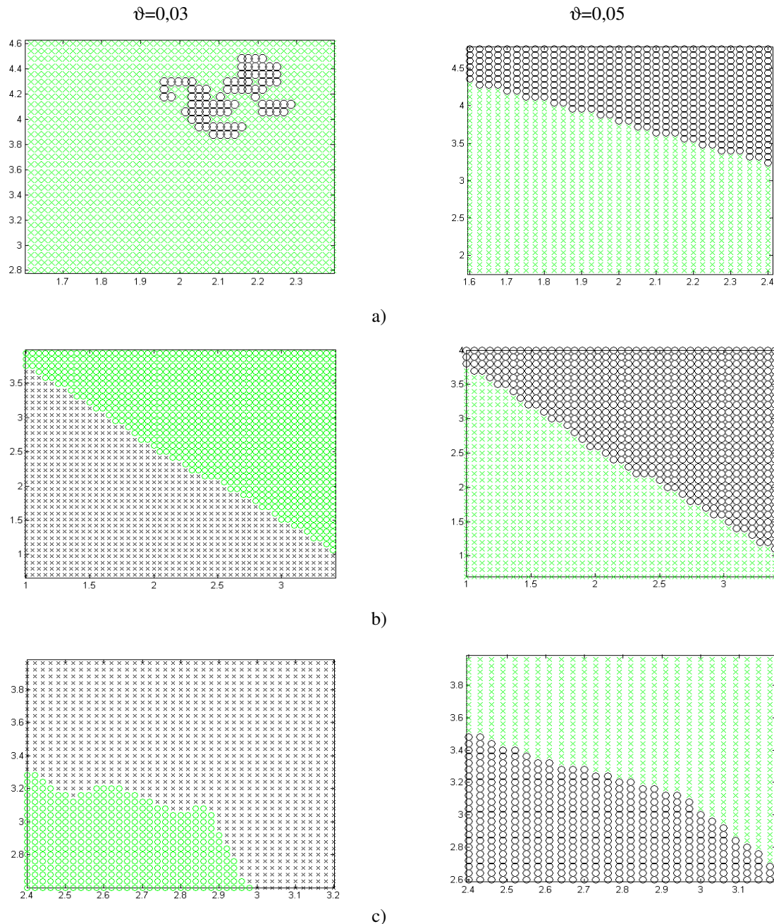
Fig. 2. The results of classification for three modes of GTE: a) m1, b) m2 and c) m3 (o – without damage S_0 , x – with damage S_1 ).
